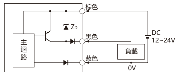
PNP
